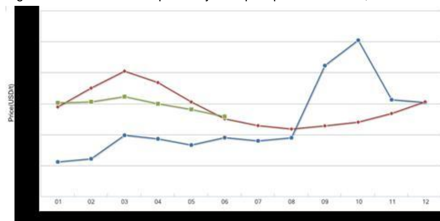
Figure 2.2.2.1-1 Ex-works price of yellow phosphorus in China, 2011-H1 2013
